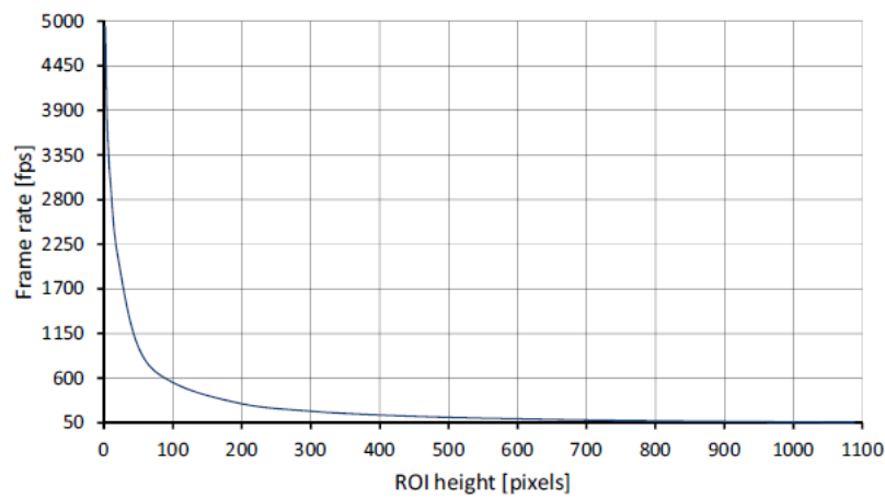
Figure 38: Frame rate as a function of ROI height
